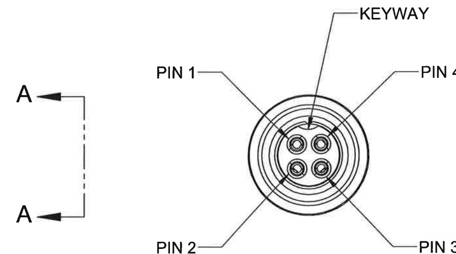
VIEW A-A SCALE 4 : 1
