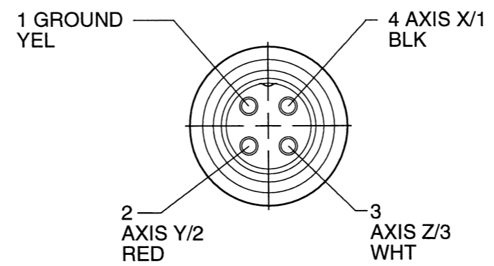
VIEW A-A SCALE 4/1
