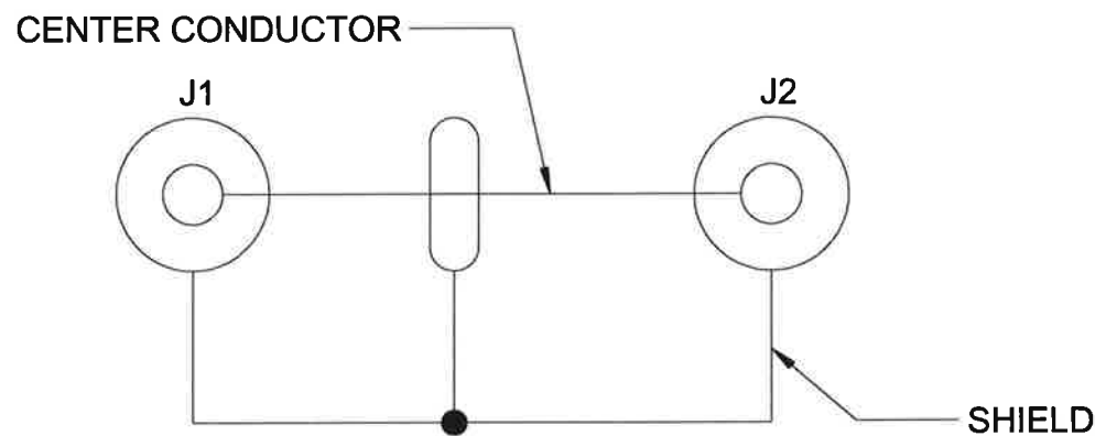
SCHEMATIC DIAGRAM
